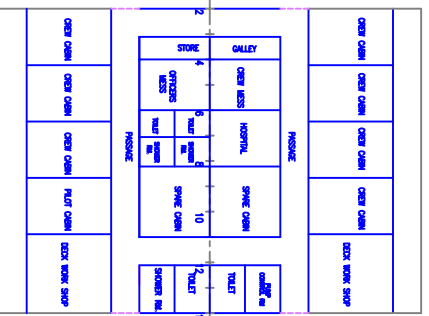
MAIN DECK ACCOMMODATION
