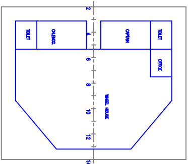
UPPER DECK W/H
