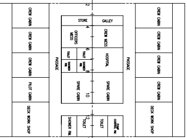
MAIN DECK ACCOMMODATION
