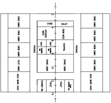
MAIN DECK ACCOMMODATION
